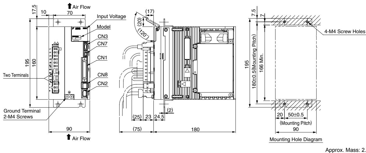
(6) Three-phase 200 VAC, Model: SGDV-120A0□A001
