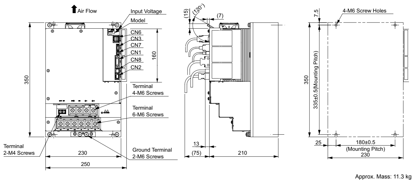
(14) Three-phase 400 VAC, Model: SGD210D1□A002000□□□ and 260D1□A002000□□□
