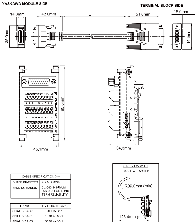
SBK-U-VBA-xx Function Chart for SGD Servo Amplifier
