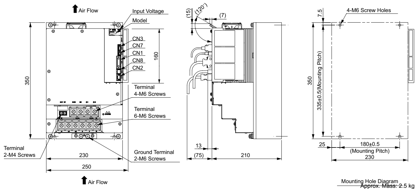
(14) Three-phase 400 VAC, Model: SGD210DE□A002000□□□ and 260DE□A002000□□□
