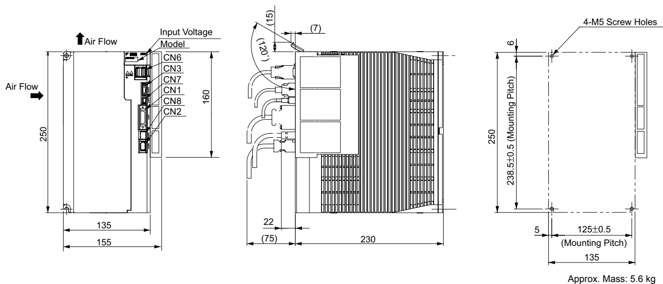
(13) Three-phase 400 VAC, Model: SGD170D1□A002000□□□
