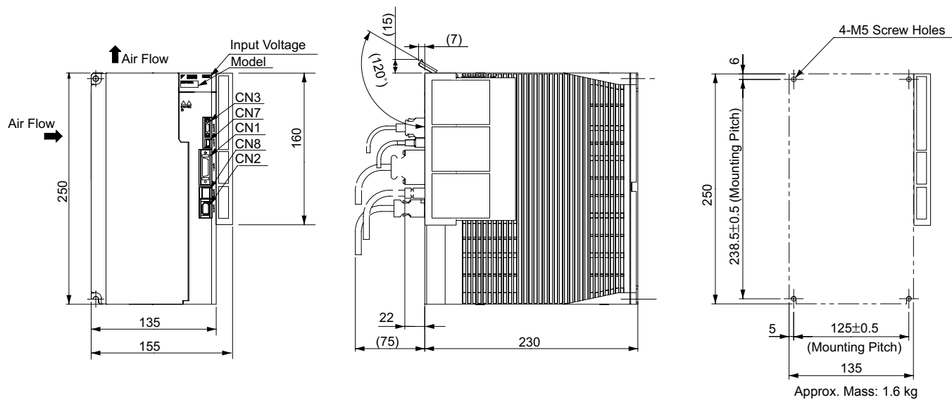
(13) Three-phase 400 VAC, Model: SGD170DE□A002000□□□
