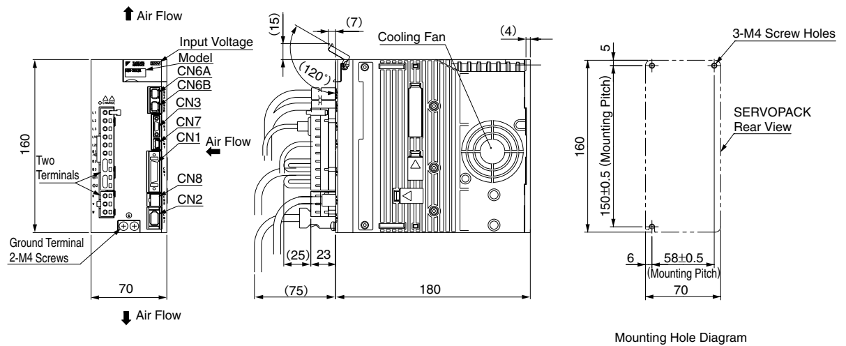
(5) Three-phase 200 VAC, Model: SGDV-3R8A2□A, -5R5A2□A, and -7R6A2□A
