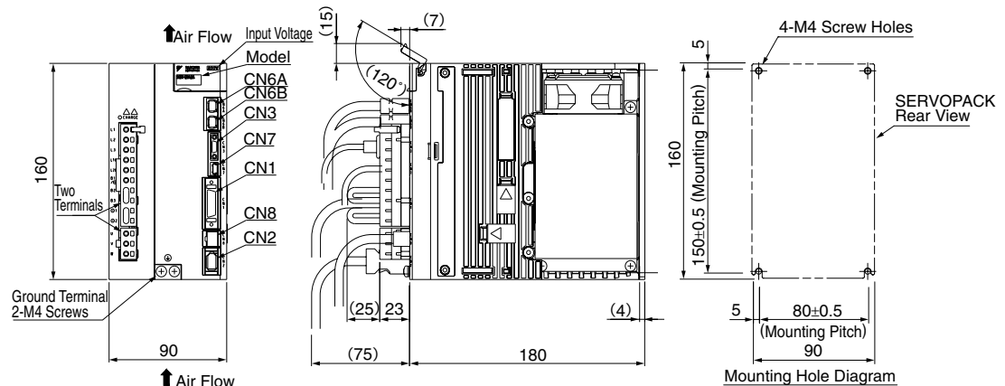
(6) Three-phase 200 VAC, Model: SGDV-120A2□A
