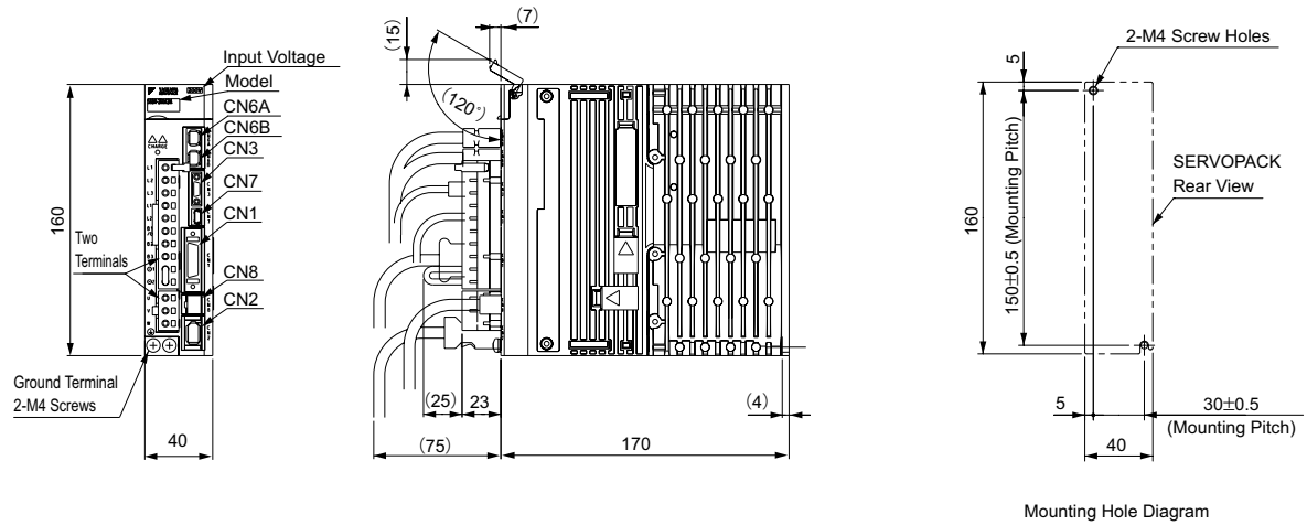
(4) Three-phase 200 VAC, Model: SGDV-2R8A2□B
