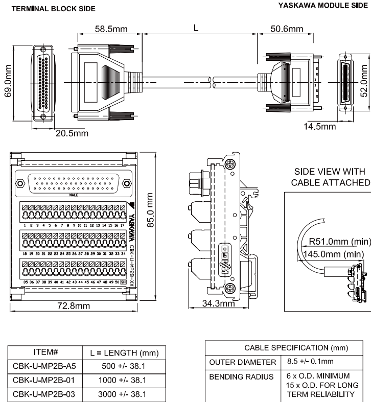
CBK-U-MP2B-XX Function Chart for MP2600iec
